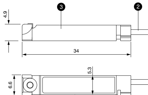
Reed Switch ( RSSQ 3210 )
